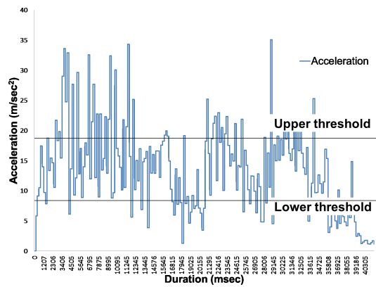
Figure 6: Running activity.
