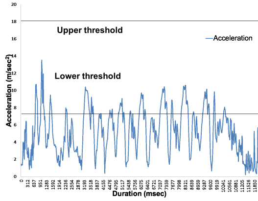
Figure 7: Walking activity.
