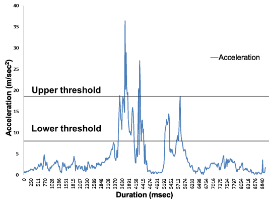
Figure 3: Strong fall.
