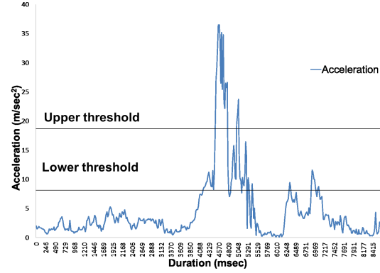
Figure 4: Sharp fall.
