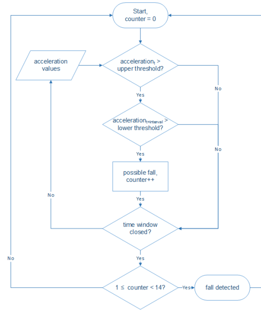
Figure 5: Fall detection algorithm.
