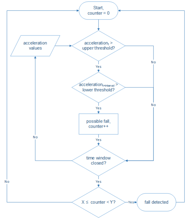
Fig. 5. Fall detection algorithm.
