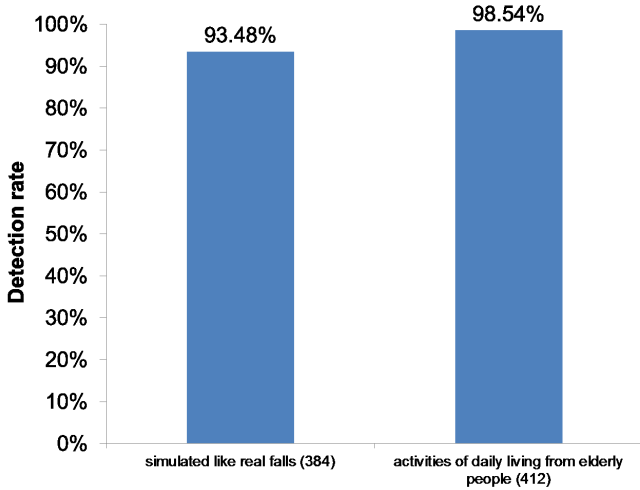
Fig. 10. Accuracy using real data from partner.
